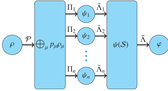
FIG. 1. Schematic picture of the deterministic coherence transformation via strictly incoherent operations. Here, \Pi_\alpha = \mathbb{P}_\alpha \cdot \mathbb{P}_\alpha for incoherent projective operator \mathbb{P}_\alpha , \psi(S) is the pure coherent state determined by \vee S , \tilde{\Lambda}_\alpha are the strictly incoherent operations such that \tilde{\Lambda}_\alpha(\psi_\alpha) = \psi , \tilde{\Lambda} is the strictly incoherent operation such that \tilde{\Lambda}(\psi) = \varphi , and all the others are the same as in the main text.
